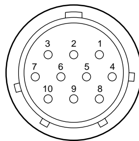
DC PARALLEL INPUT
