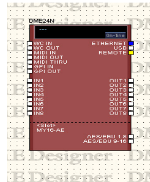
DME24N with an I/O card installed in its expansion slot.
